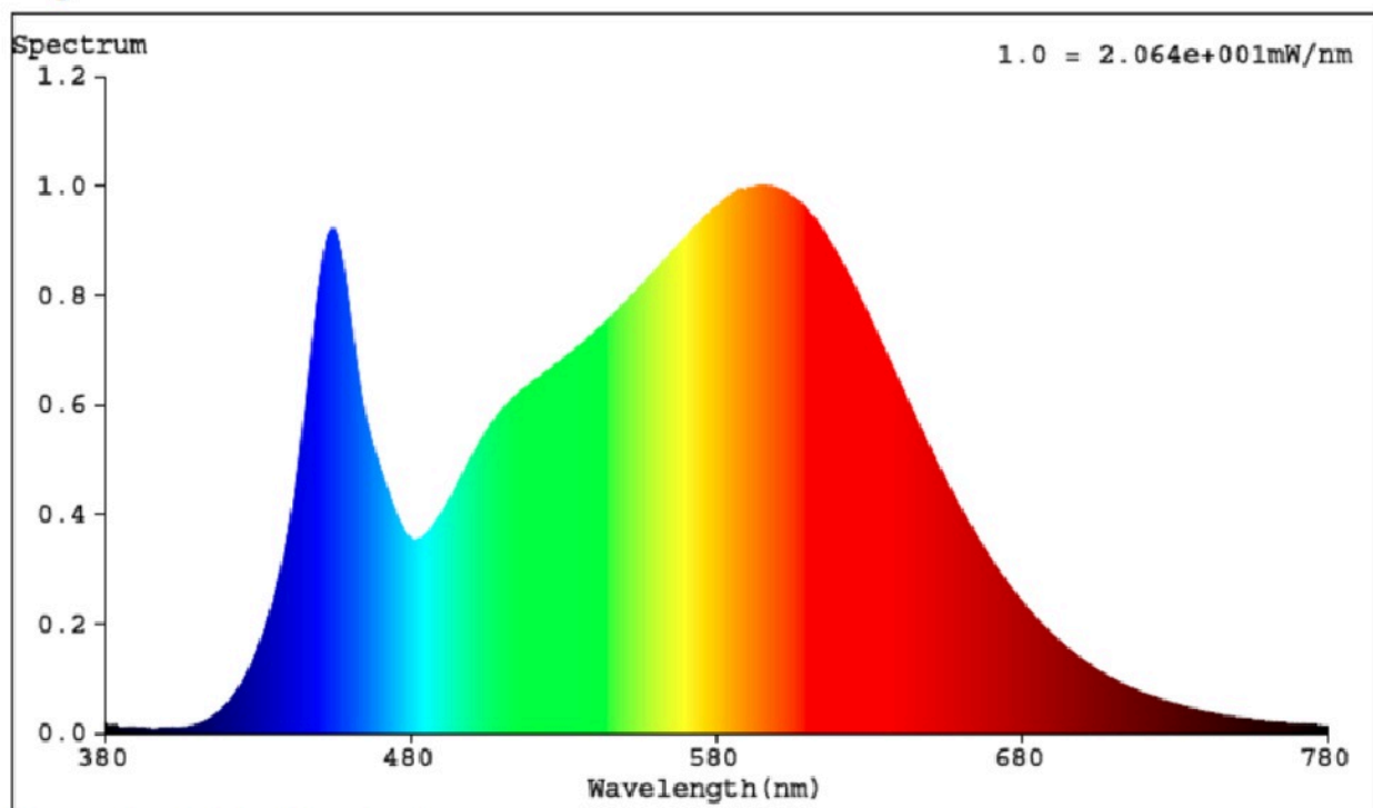
Spectral Distribution
